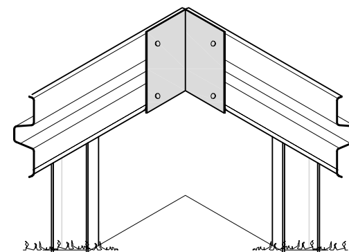
Binnenhoek oplossing
