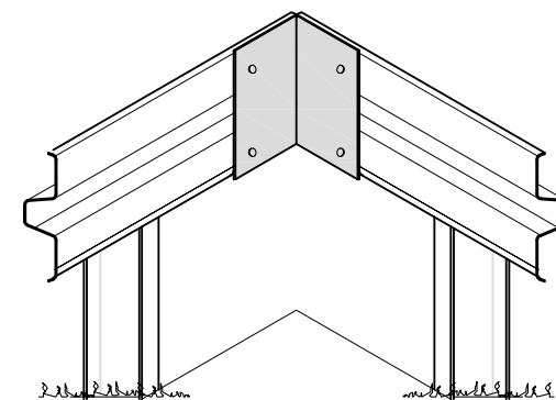
Binnenhoek oplossing
